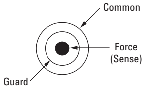
Figure 4.4. SMU terminal
