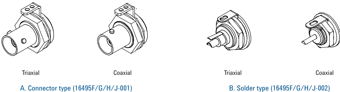
Figure 5.5. Connection type of connector plate (rear)
