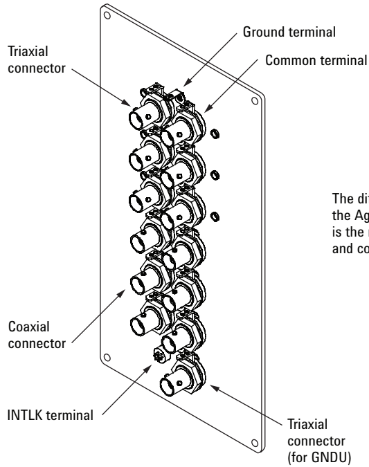
Agilent 16495H-001
