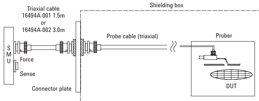
Figure 4.6. Examples of a SMU non-Kelvin connection
