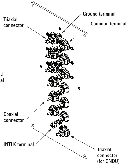
Agilent 16495H-002
