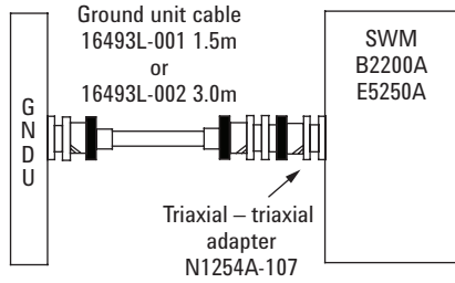
Figure 3.2. Examples of a GNDU non-Kelvin connection to SWM
